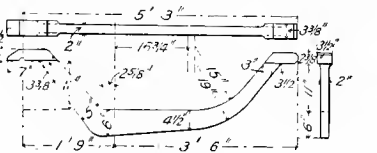
Figs. 5064-66. TRACK EQUALIZER.
